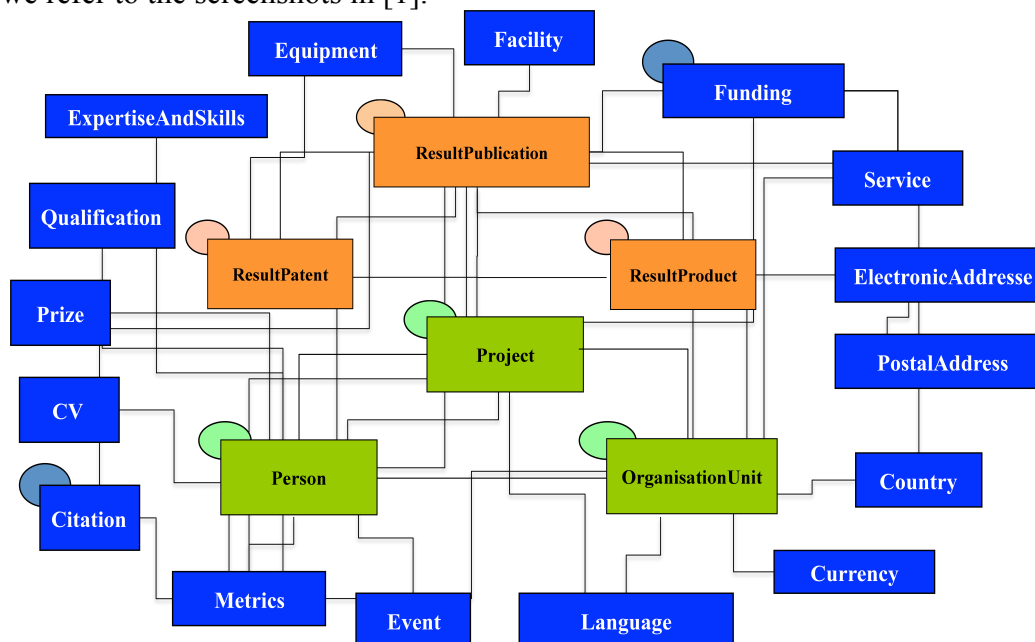
Figure 1: CERIF 2008 – 1.1 entities and some relationships
