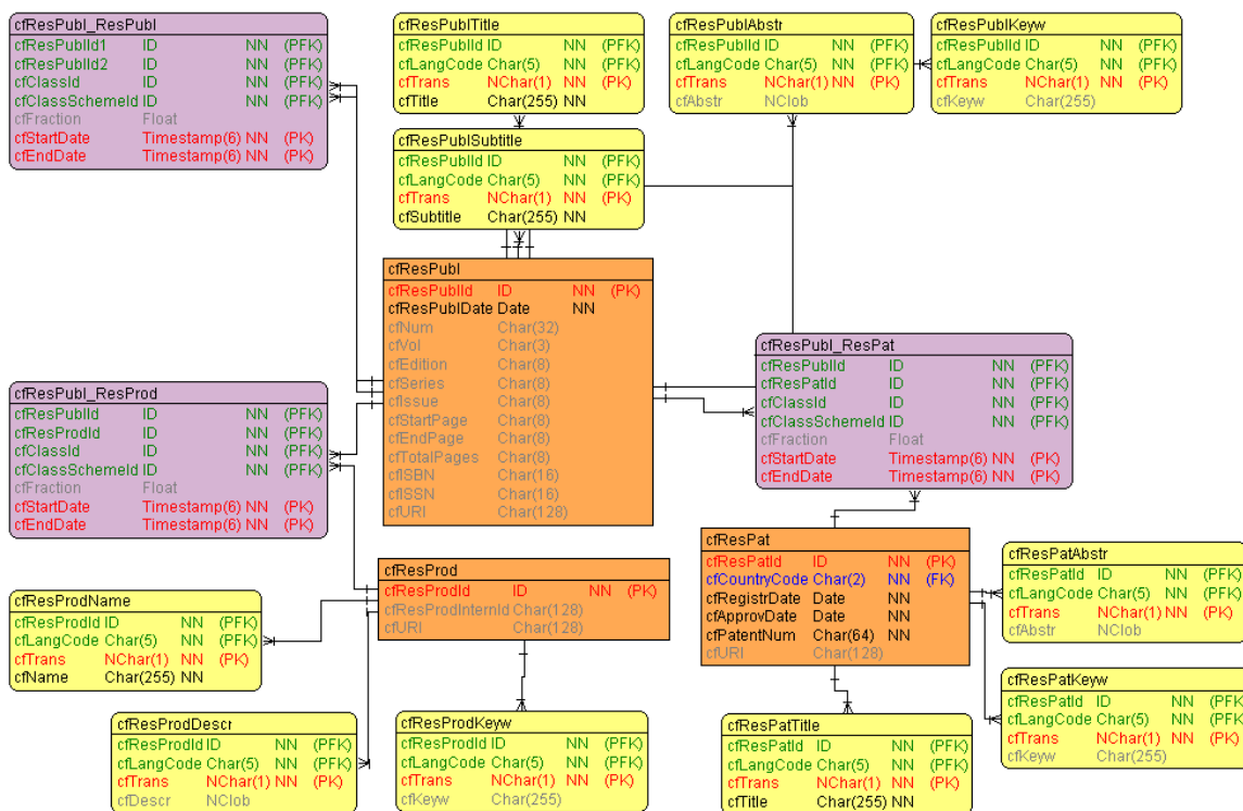
Figure 8: CERIF Result Entities, their Recursion and some Link Entities
